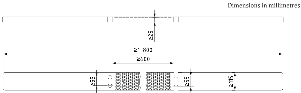
Figure 3 — Pilot ladder spreader step and replacement spreader step construction, hole and slot types for side ropes
